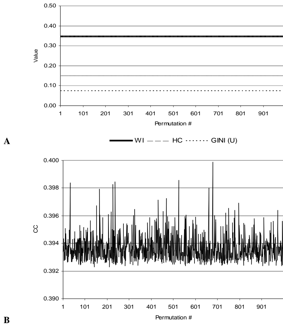
Fig. 2. Results of permutation tests (Test 2: restricted test) for selected inequality measures - WI, HC, and Gini (U) (A) and CC (B)
